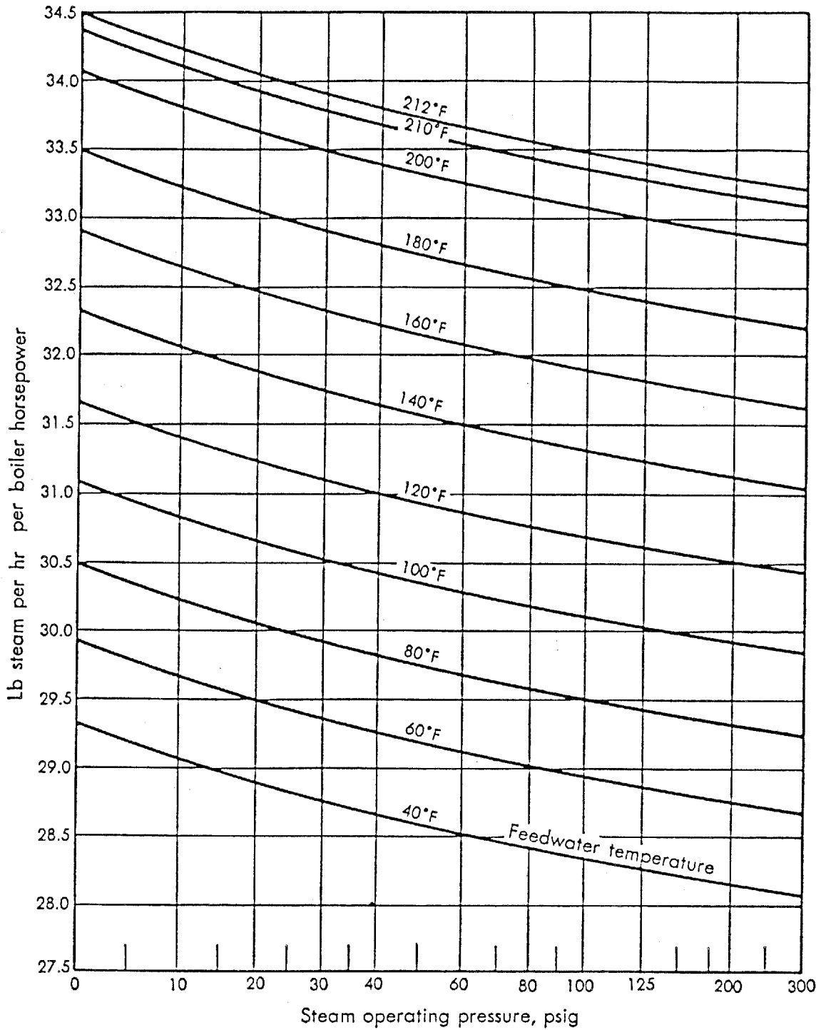
FIG. 1 EQUIVALENT EVAPORATION RATES
